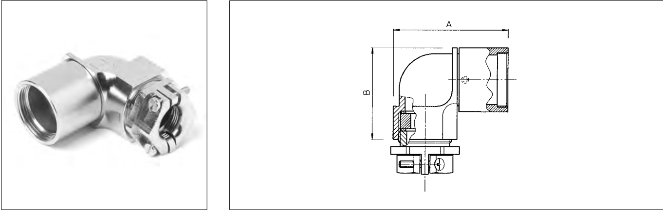
Metal right angle cable clamp with strain relief nut (UTG--LPGN / UT0--LPGN)
