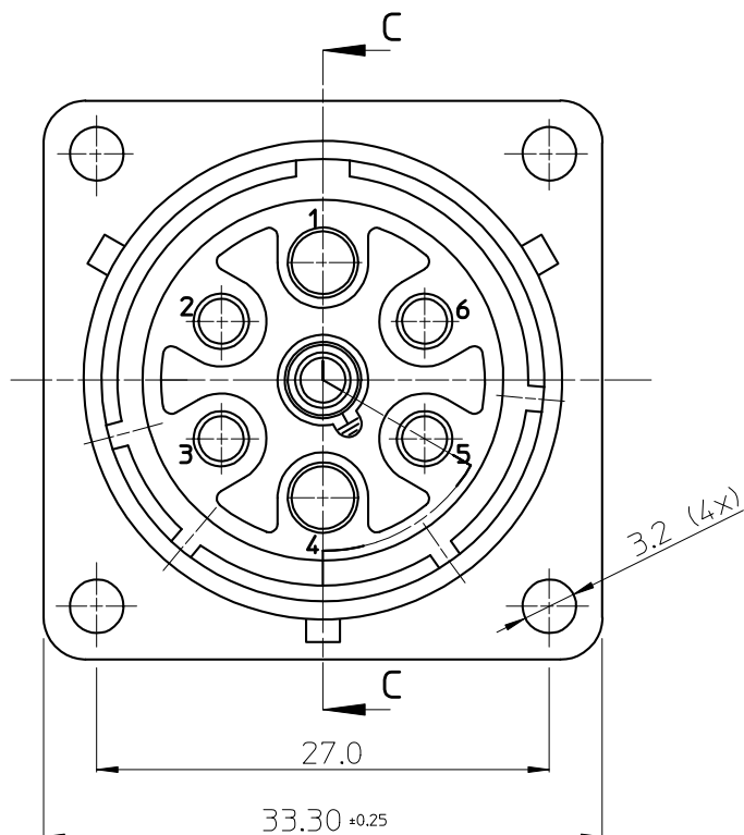
MATING FACE
